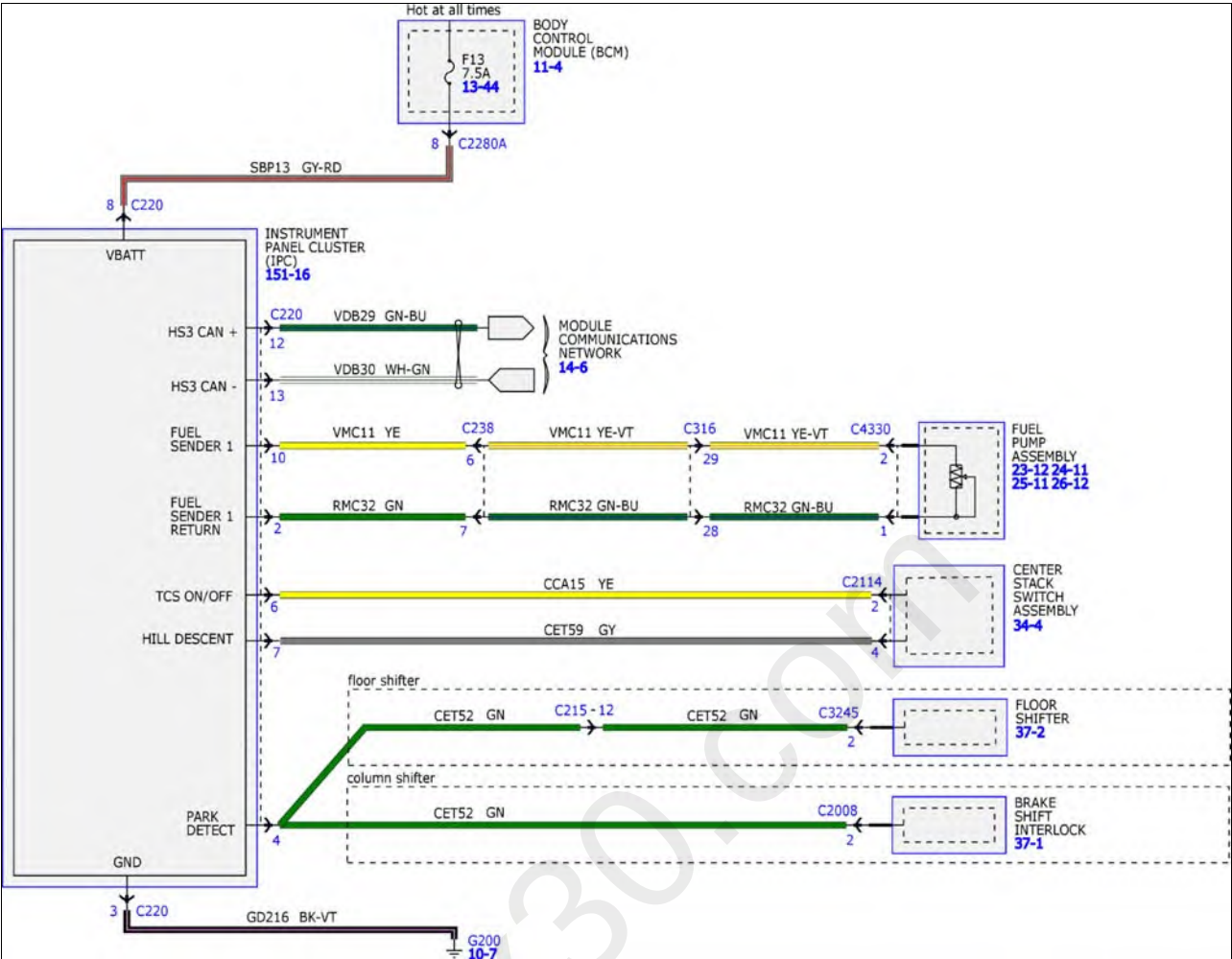
Fig 1: Instrument Cluster System Wiring Diagrams (1 Of 2)
