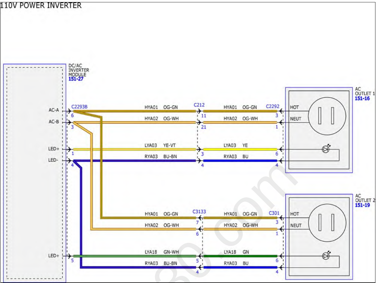
Fig 4: Horn/Cigar Lighter System Wiring Diagrams (4 Of 4)
